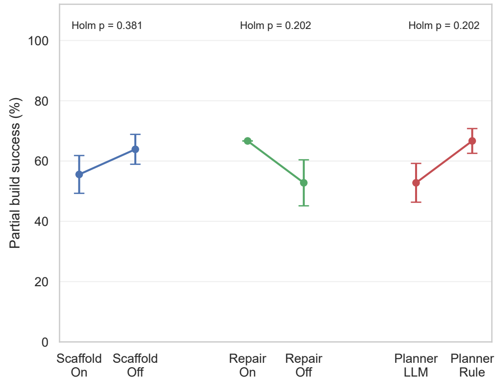
(a) Automatic partial build success
