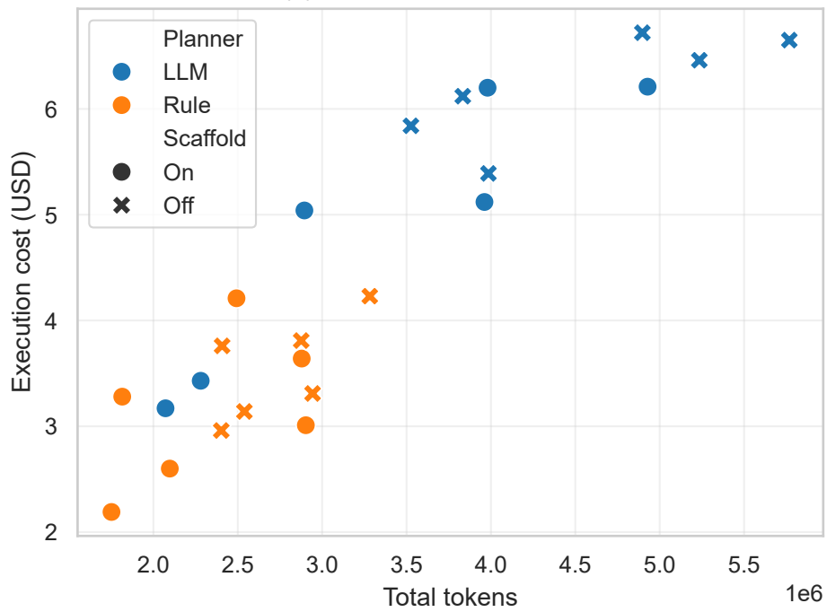
(b) Tokens and execution cost
