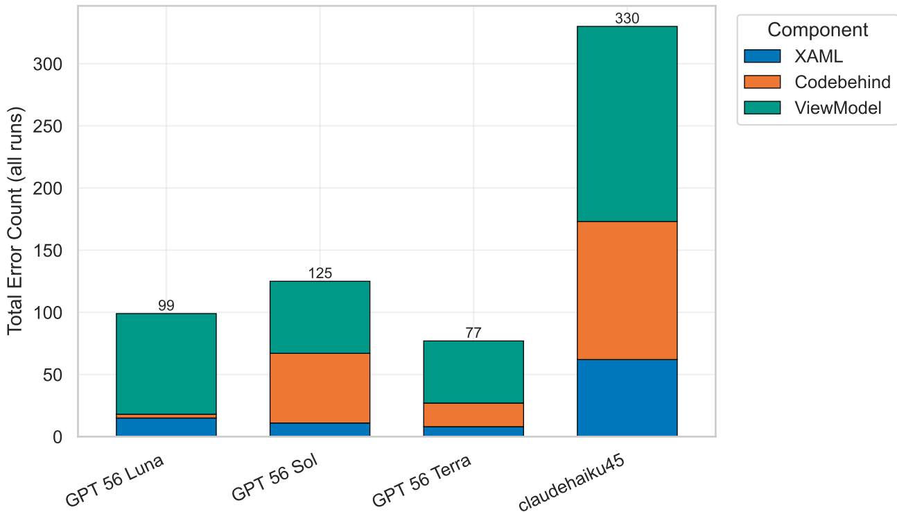
Component Error Distribution by Model (XAML / Codebehind / ViewModel)
