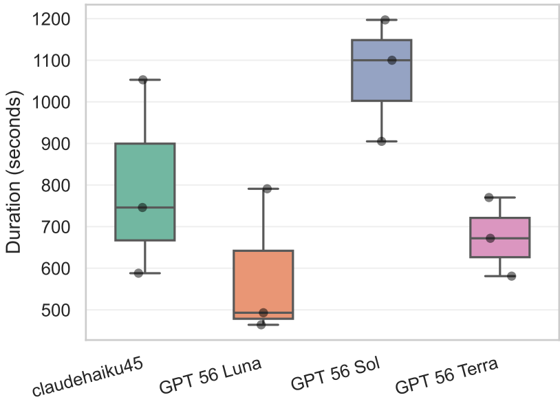
Migration Duration by Model
