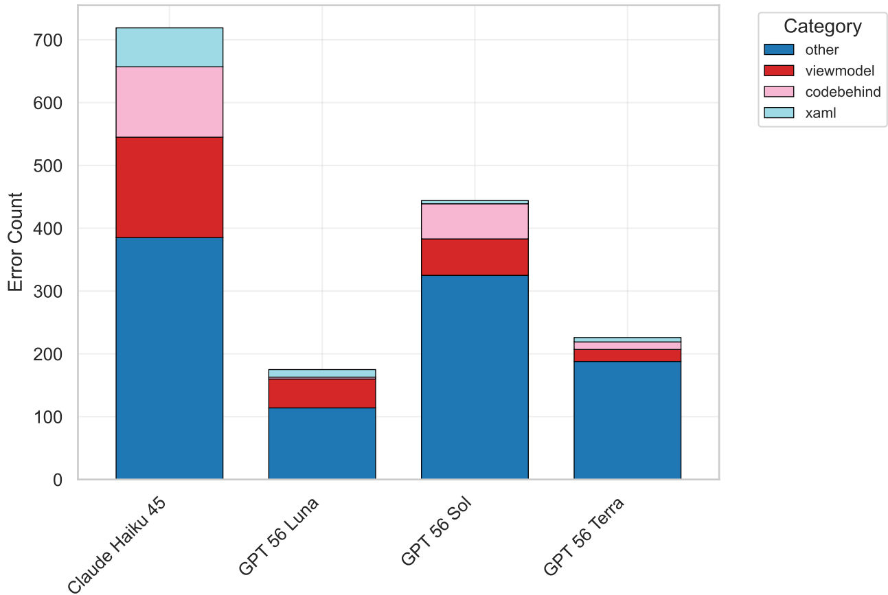
Error Category Distribution by Model
