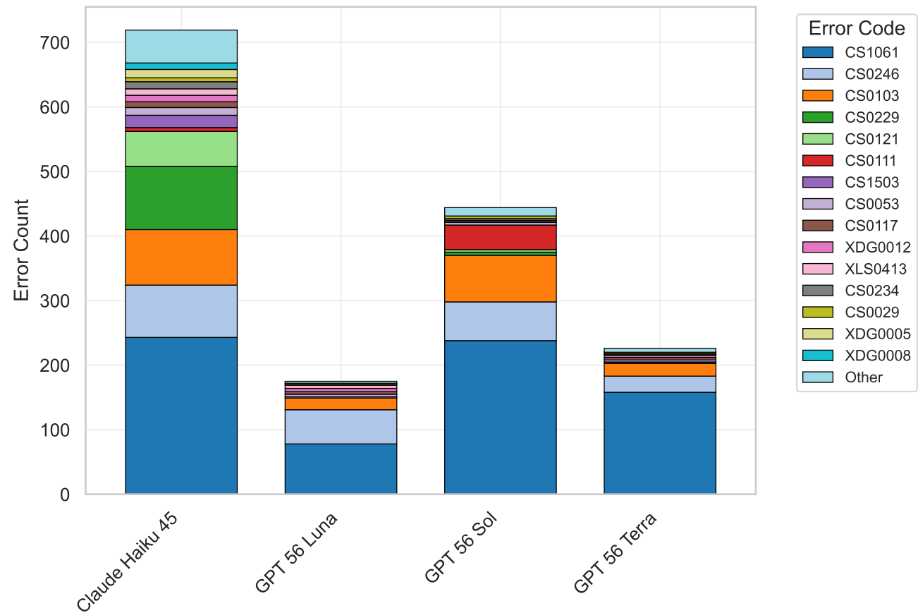
Error Code Distribution by Model
