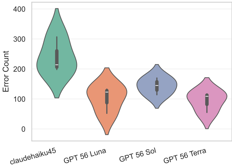
Error Distribution by Model
