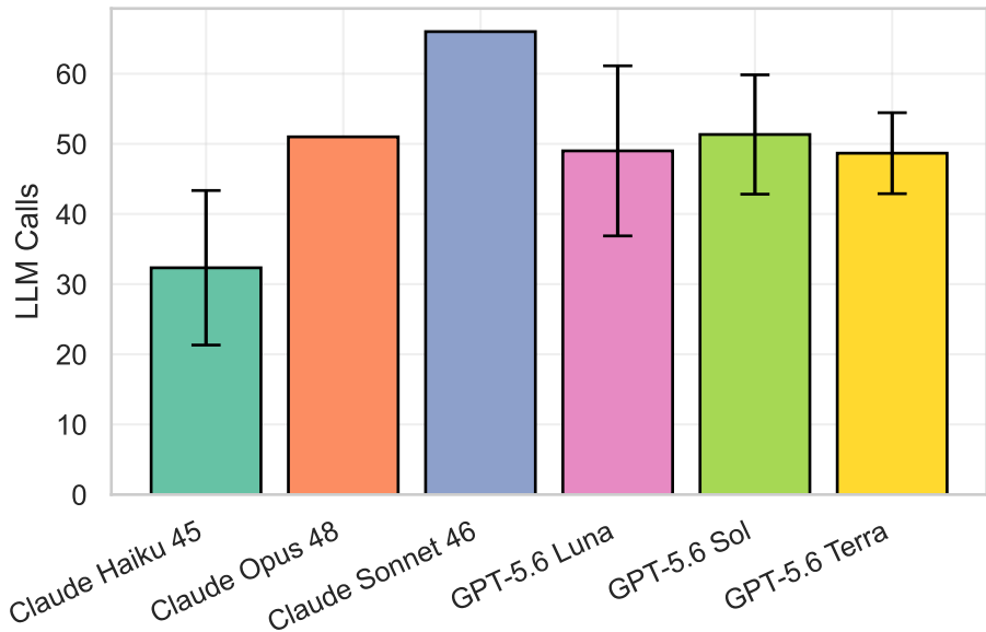
Mean LLM Calls by Model ( \pm SD)
