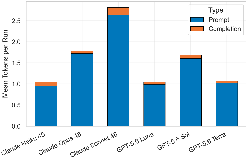
Token Composition by Model (Prompt vs. Completion)
