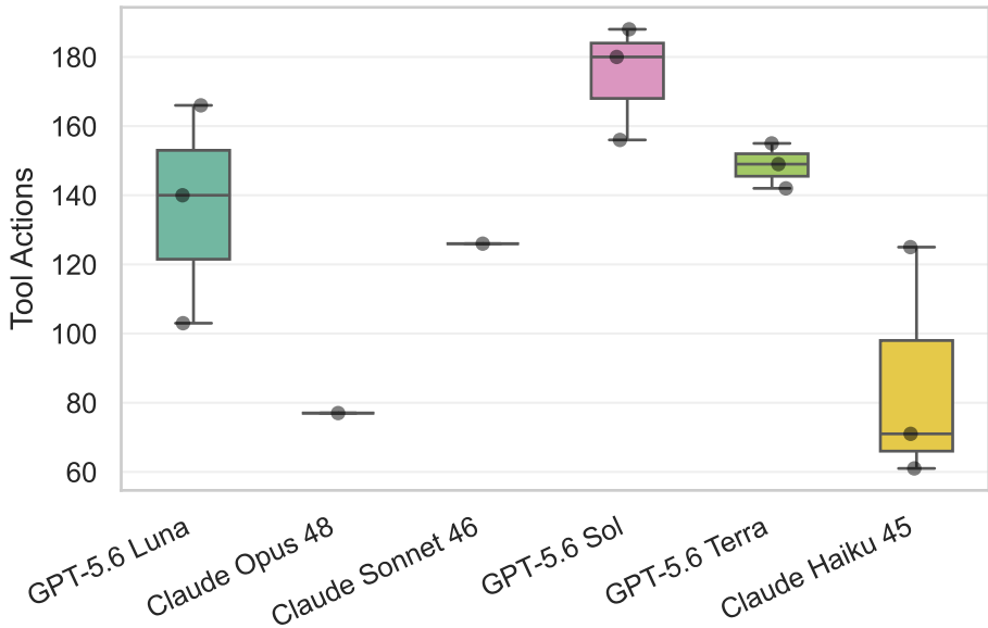
Total Tool Actions by Model
