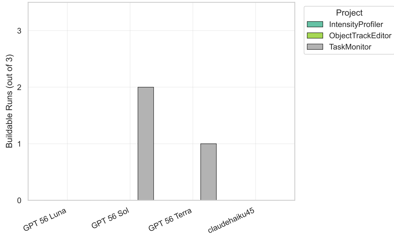
Successful Project Builds by Model
