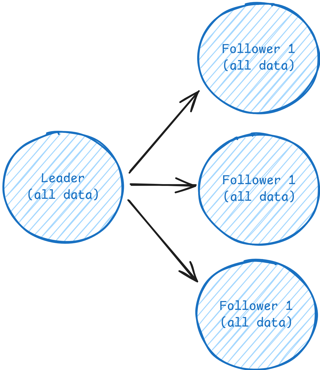
Leader-Follower Replication
