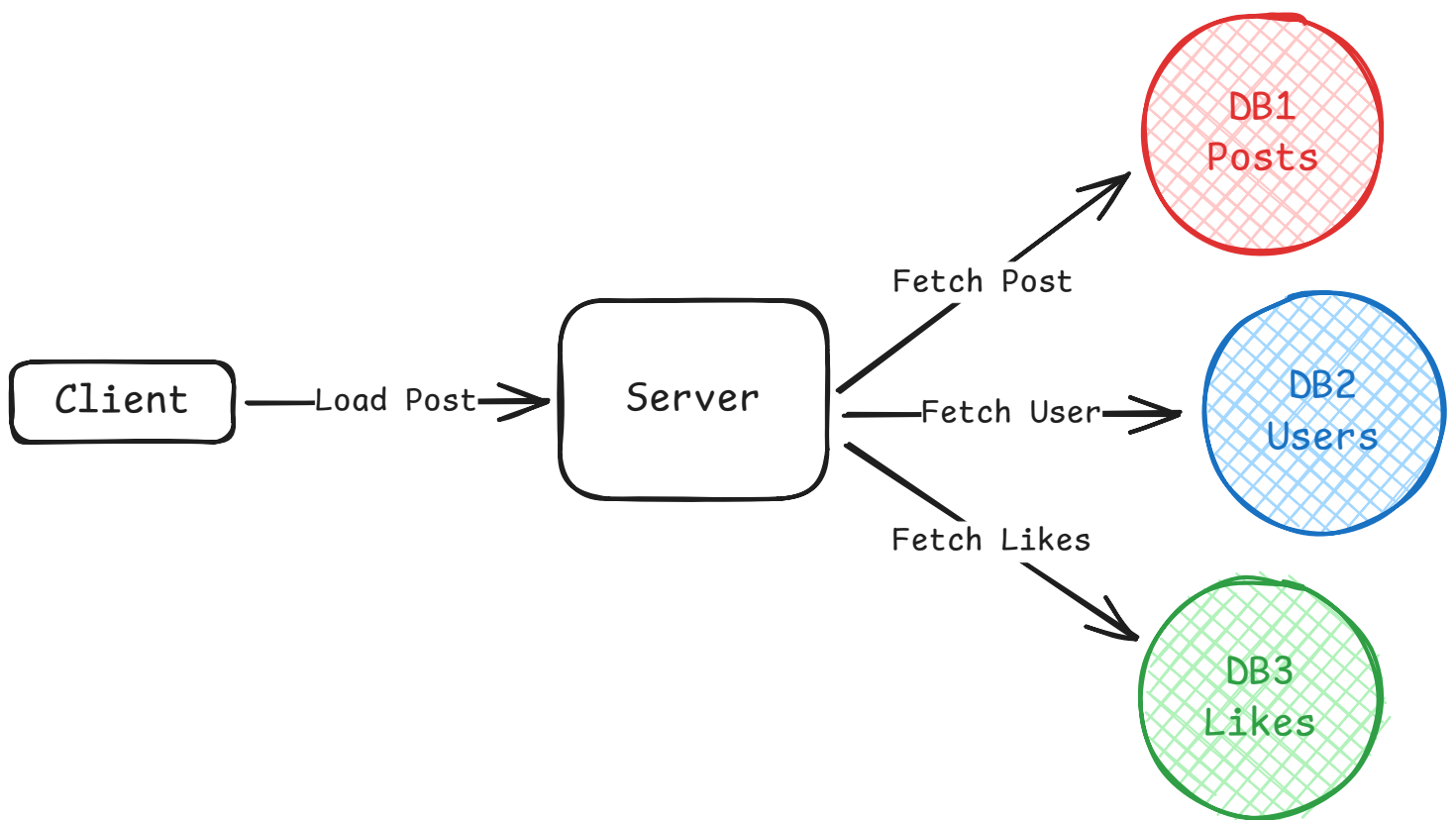
Functional Sharding
