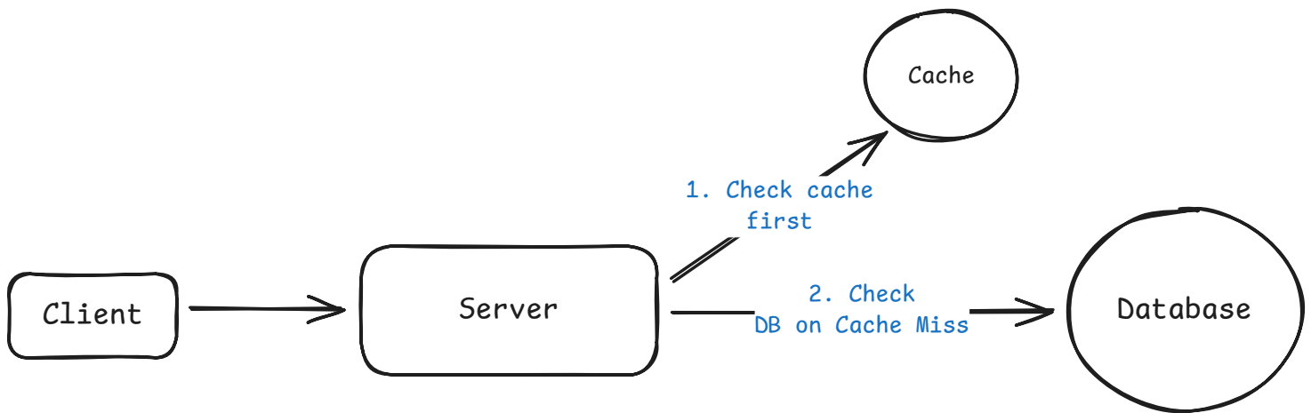
Application-Level Caching
