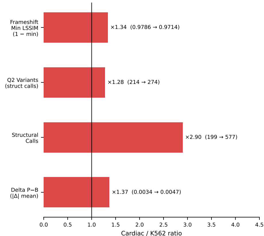
C Cardiac vs K562 Amplification
