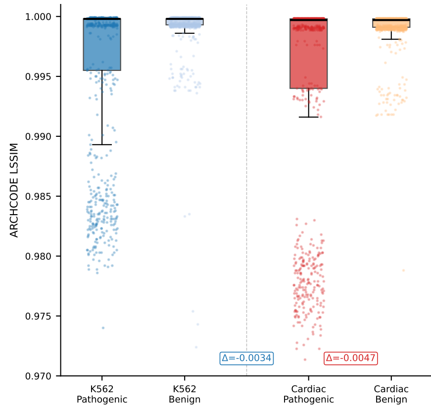
A LSSIM Distribution: K562 vs Cardiac
