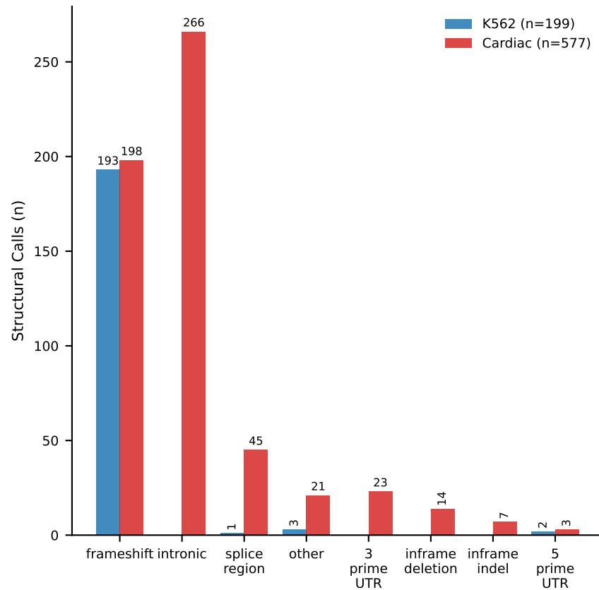
B Structural Calls by Category
