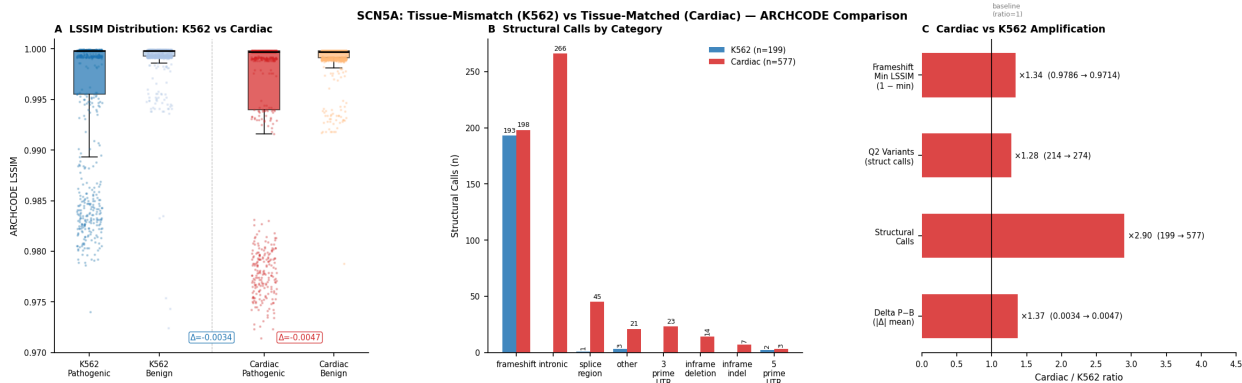
Figure 6: SCN5A tissue-match experiment: K562 (Class E) versus cardiac (Class B). (A) LSSIM distribution for pathogenic and benign variants under both configurations. (B) Structural calls by variant category. (C) Amplification ratios showing 1.37\times delta, 2.90\times structural calls, and 1.28\times Q2 variants.
