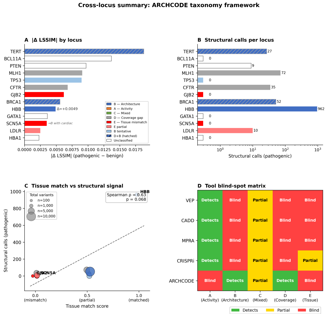
Figure 8: Cross-locus summary of ARCHCODE taxonomy framework. (A) |\Delta \text{LSSIM}| (pathogenic minus benign) by locus, colored by taxonomy class assignment. TERT shows the largest absolute delta; HBB shows the strongest Class B signal. (B) Structural call counts per locus (log scale). HBB dominates with 962 calls. (C) Tissue match score versus structural calls: HBB (tissue match = 1.0) is the clear outlier with Spearman \rho = 0.63 . (D) Tool blind-spot matrix: only ARCHCODE detects Class B (architecture-driven); all sequence-based tools (VEP, CADD, MPRA, CRISPRi) are blind to this class.
