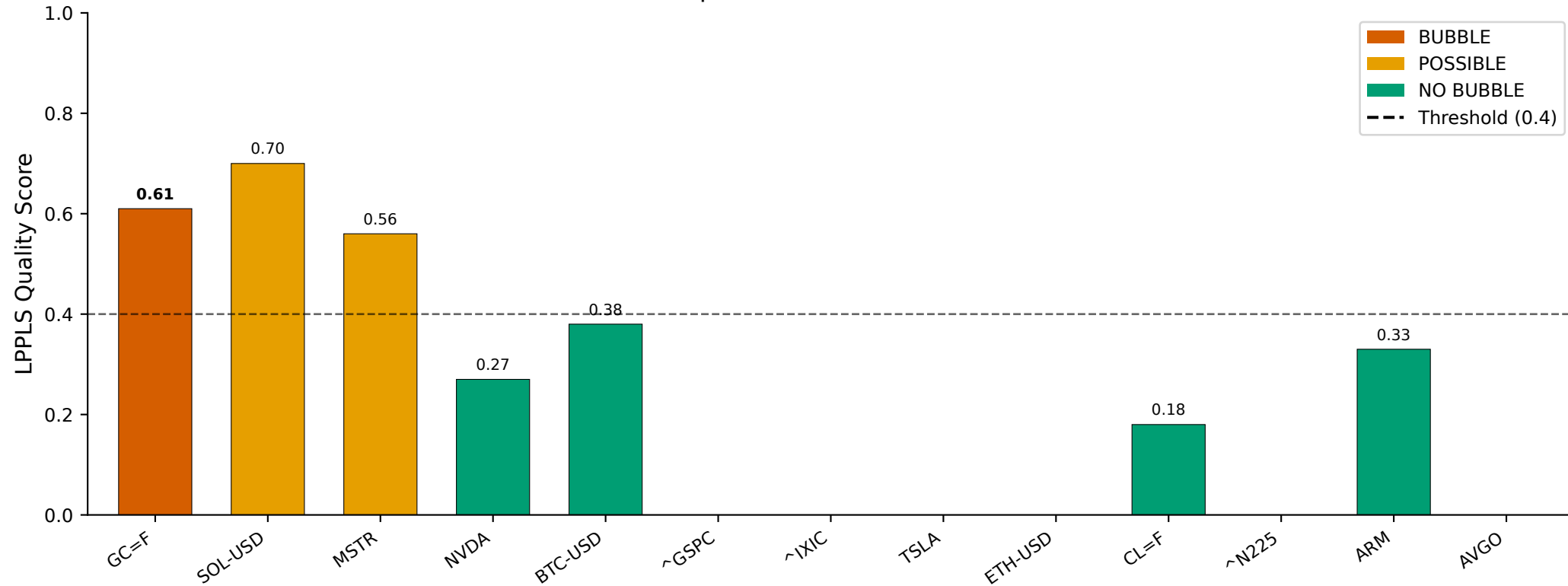
PhaseBreak v2 — April 2026 Forward Predictions (13 assets)
