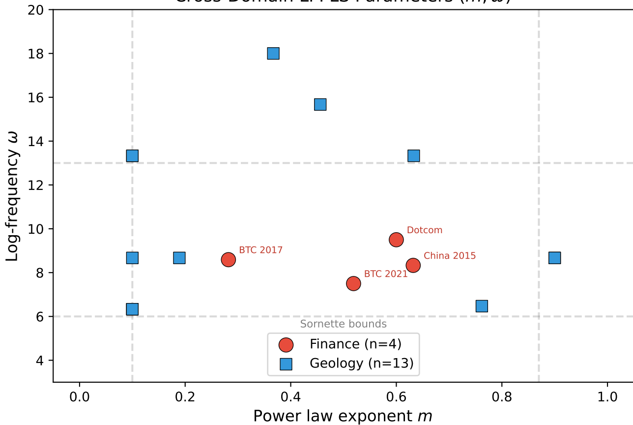
Cross-Domain LPPLS Parameters ( m, \omega )
