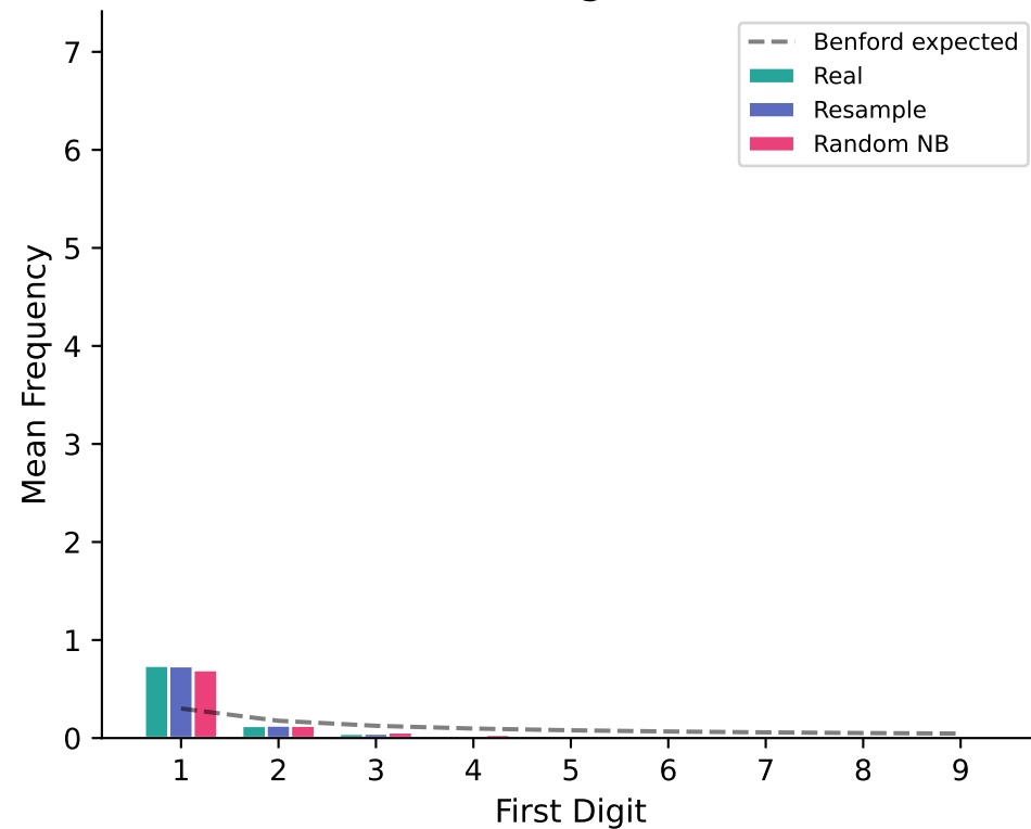
A. Mean First-Digit Distribution
