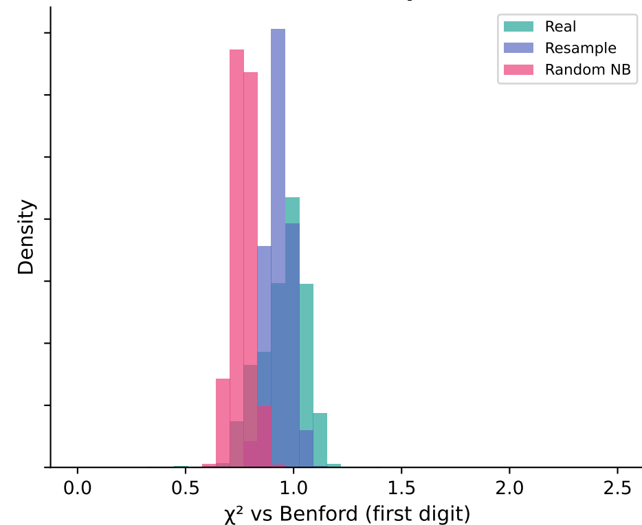
C. Chi-Squared Divergence from Benford Expected
