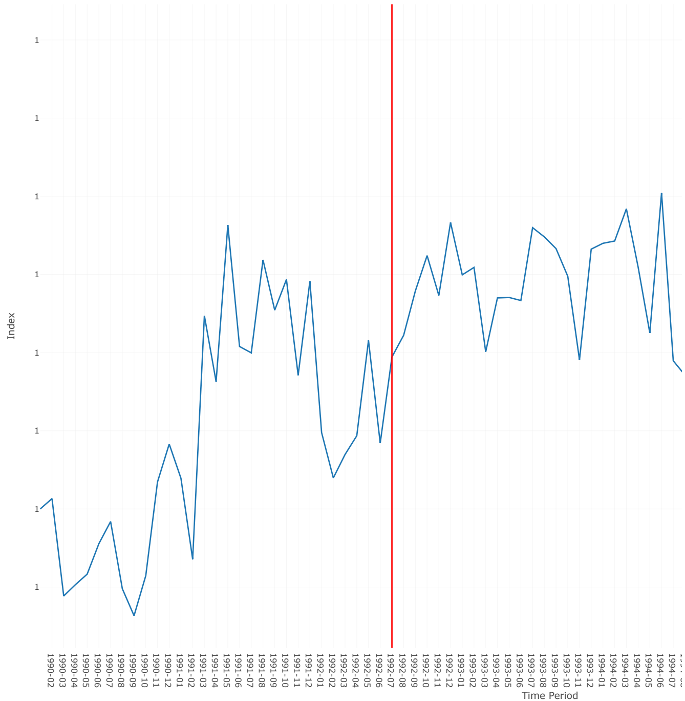
CCDI with mean splice (Fabric Softeners category)
