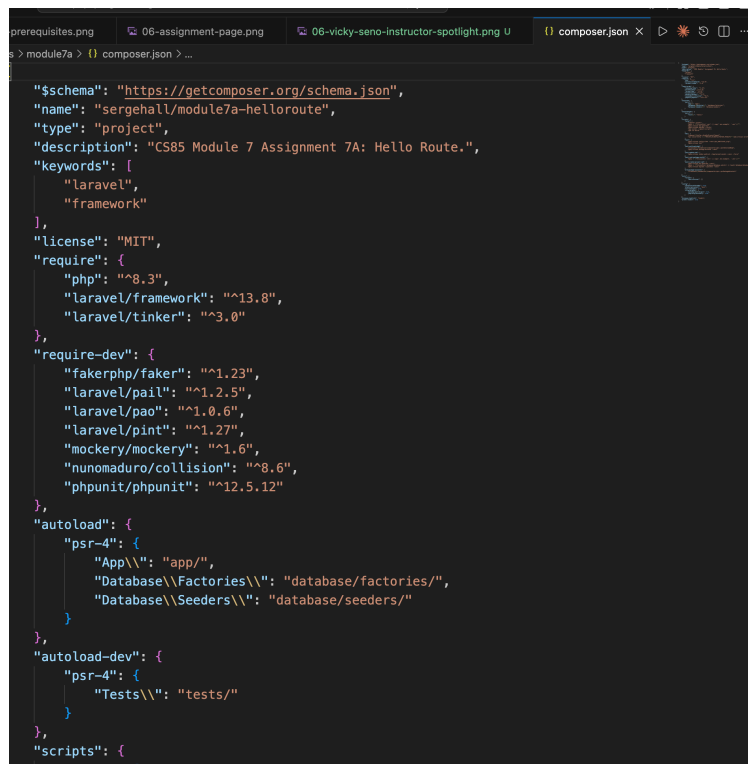
Figure 2. Module 7A composer.json showing the Laravel framework dependency and project configuration.
