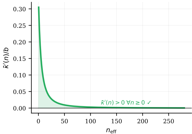
(b) Double prudence: \partial^2 f^{\text{BGZ}}/\partial d \partial n = \bar{\kappa}'(n)/b > 0
