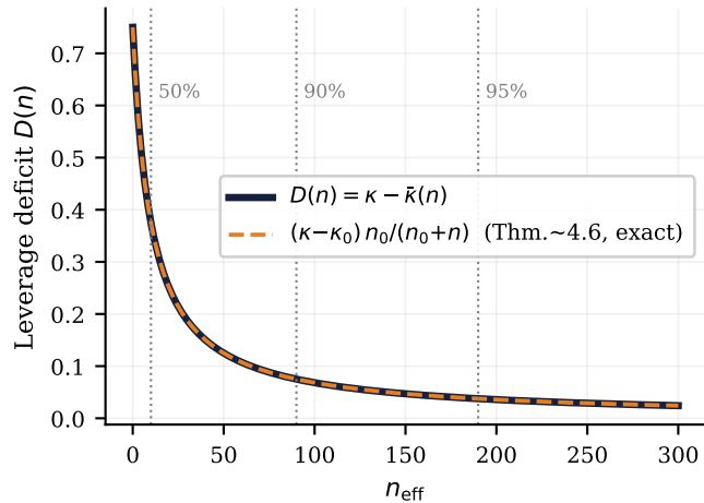
(a) Exact O(1/n) convergence to oracle (Bayes GZ rule)
