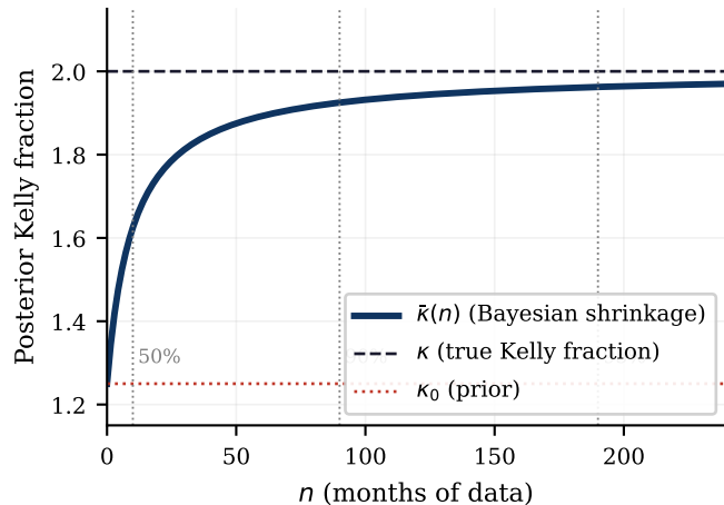
(a) Shrinkage trajectory \bar{\kappa}(n) from prior \kappa_0 to oracle \kappa
