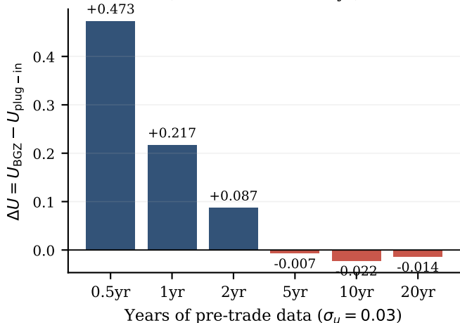
(b) Bayes GZ advantage by horizon (crossover at n \approx 3 yr)
