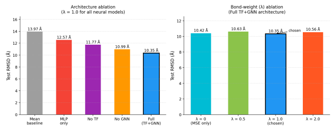
FIG. 5. Ablation study summary. Left: test RMSD for all five architecture variants. The full Transformer + GNN model (black border) achieves the lowest RMSD (10.35 Å), outperforming the mean-distance baseline by 3.6 Å. Right: test RMSD for four bond-constraint weights \lambda using the full architecture. \lambda = 1.0 (black border) achieves the best RMSD of 10.35 Å.
