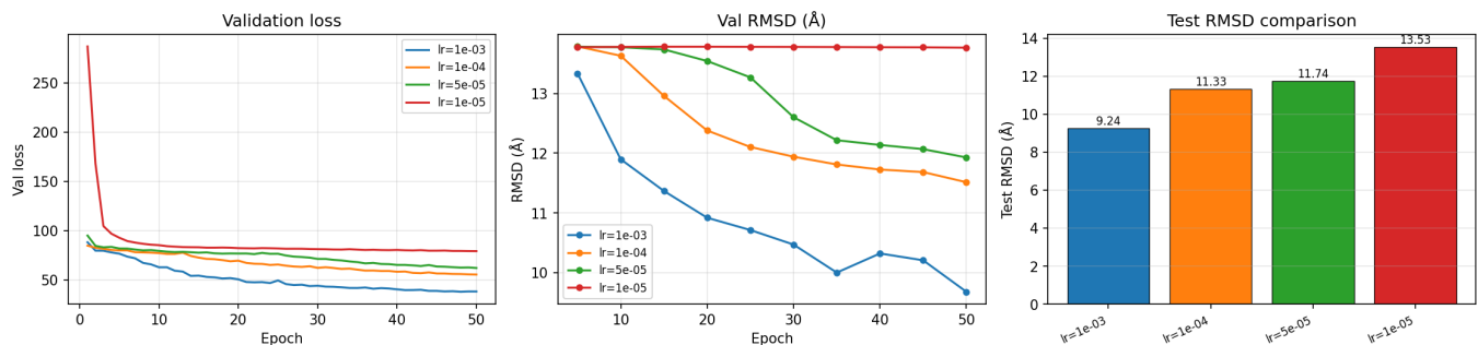
FIG. 6. Learning-rate ablation over 50 epochs. Left: validation loss curves. Centre: validation RMSD every 5 epochs. Right: final test RMSD. A learning rate of 10^{-3} converges fastest and achieves the best test RMSD of 9.24 Å.
