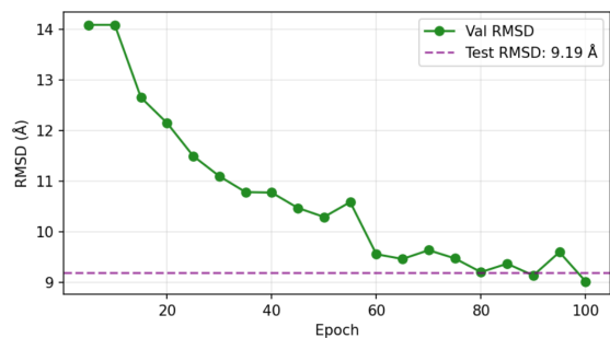
FIG. 3. C_\alpha RMSD after MDS and Kabsch alignment. Validation RMSD decreases during training after 3D reconstruction with MDS and structural alignment with the Kabsch algorithm.
