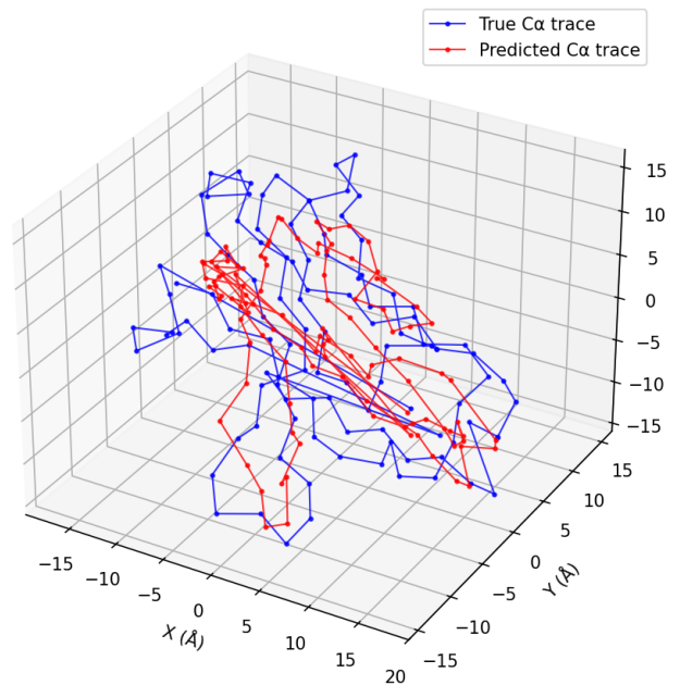
FIG. 8. C \alpha protein structure prediction for 10ZO chain A. Comparison between the ground-truth and predicted C \alpha backbone structures.
