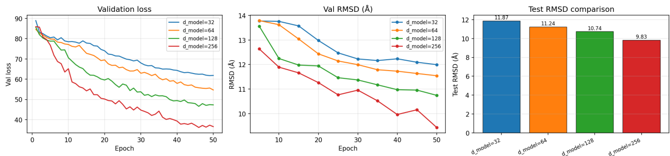
FIG. 7. Embedding-dimension ablation over 50 epochs. Left: validation loss curves. Centre: validation RMSD every 5 epochs. Right: final test RMSD.
