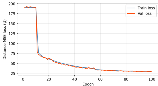
FIG. 2. Training and validation loss curves. MSE loss decreases over 100 epochs for both training and validation sets.
