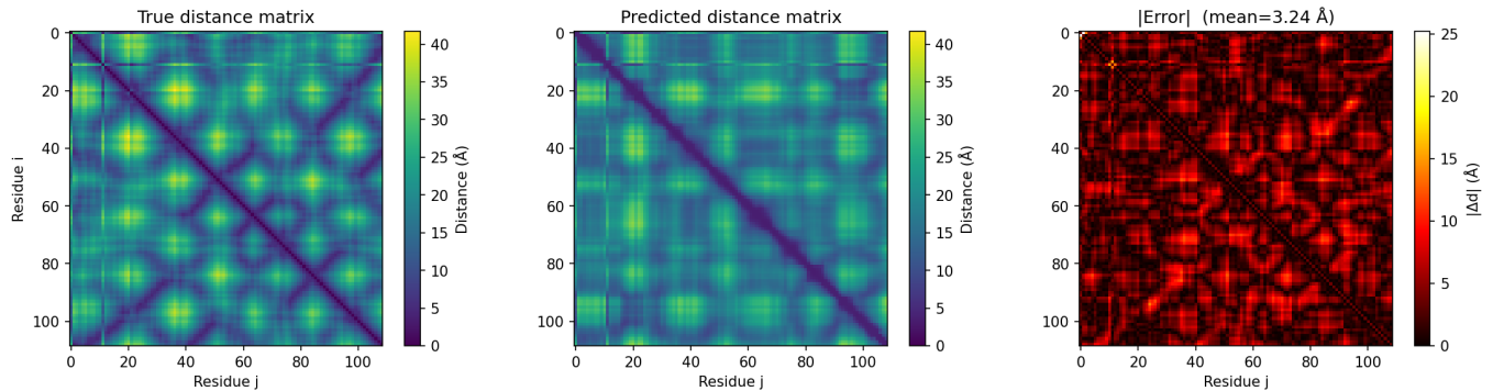
FIG. 4. C \alpha distance matrix prediction for 10ZO chain A. True and predicted C \alpha distance matrices are compared for residues i and j . The error map shows the absolute distance error, with a mean error of 3.24 Å; brighter regions indicate larger discrepancies.
