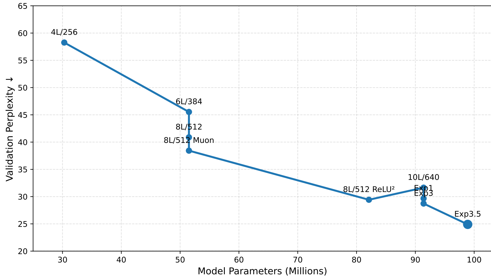
Validation Perplexity Across Model Scaling and Optimization Stages
