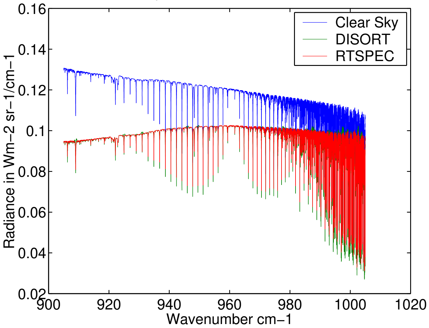
kCARTA Spectrum for DownLook Instrument
