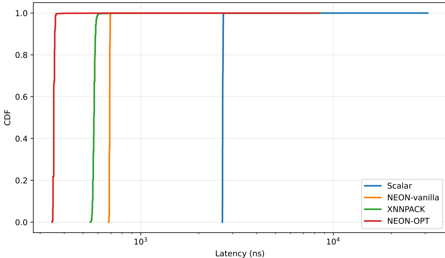
MLP inference latency across kernels
