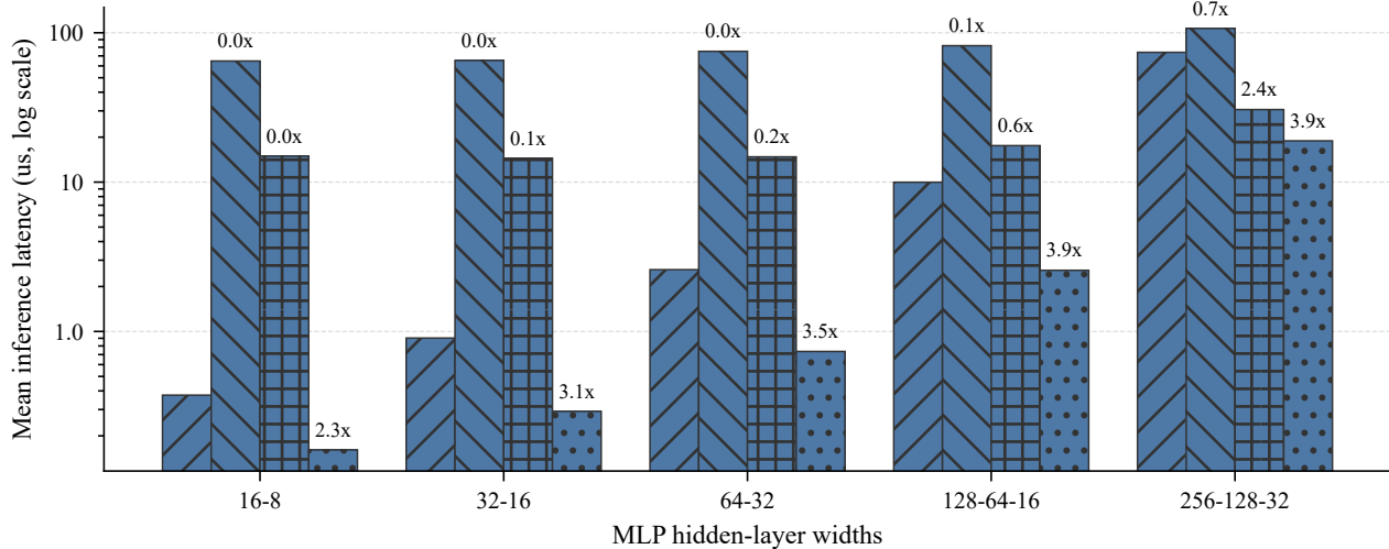
BF3 ARM (A78): all kernels
