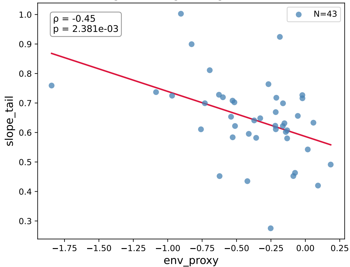
High-mass regime ( \log M \geq 10.6 )
