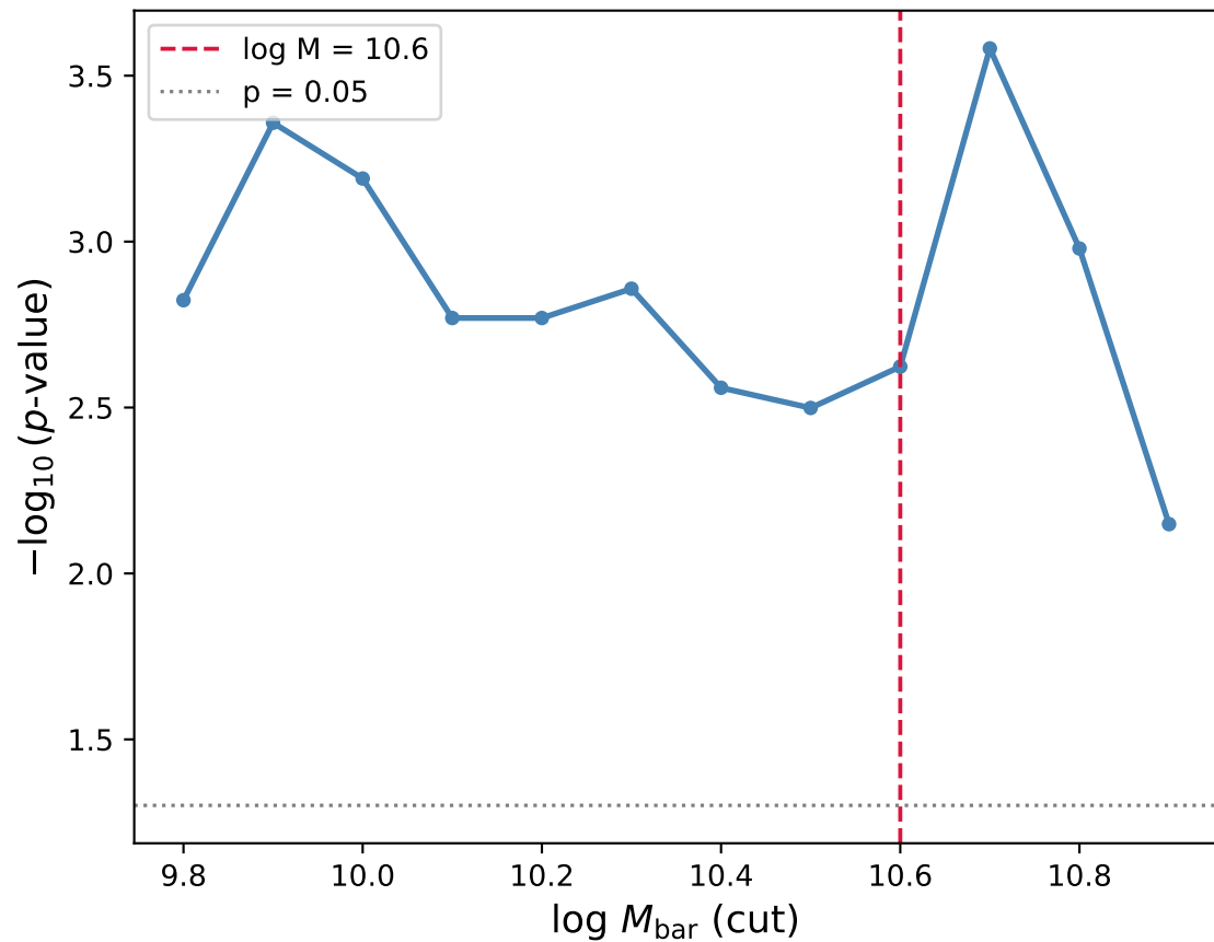
Mass-threshold scan
