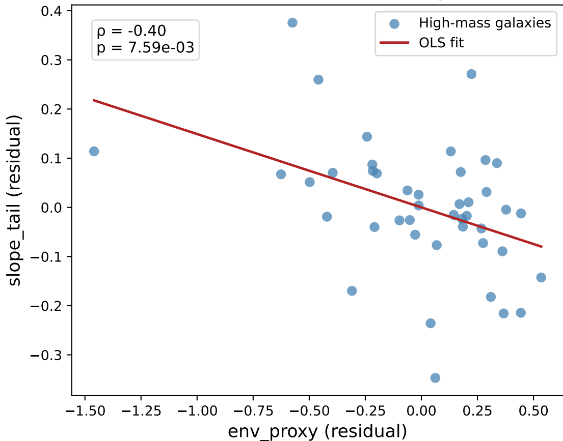
Residual environmental correlation (high-mass)
