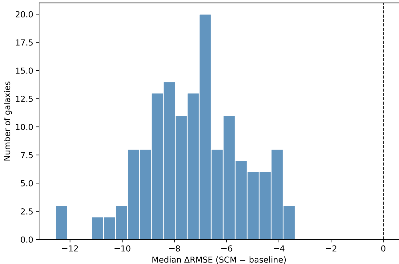
Distribution of \Delta\text{RMSE} per galaxy (OOS)
