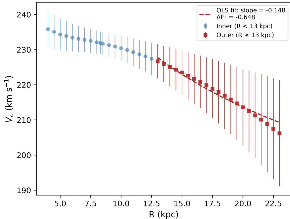
Milky Way — Cepheid rotation curve
