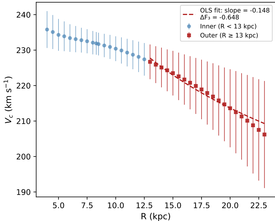
Milky Way — Cepheid rotation curve
