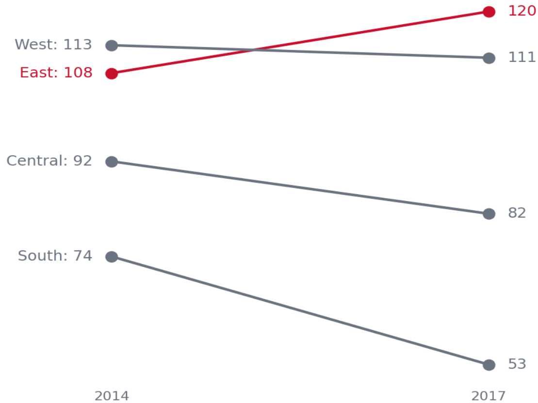
Slopegraph — Sales por Region: 2014 vs 2017
