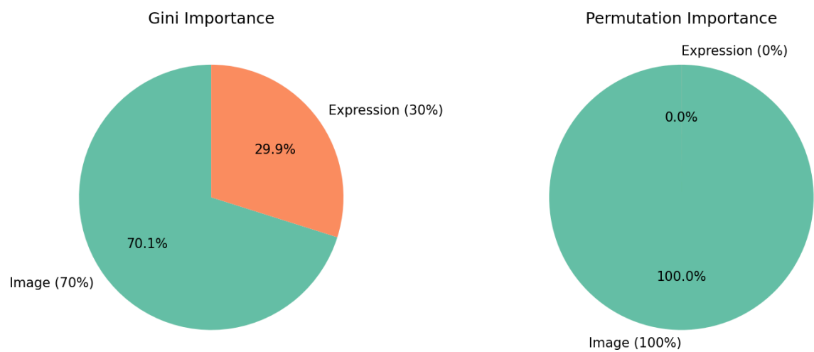
Figure 2: Importance by Modality
