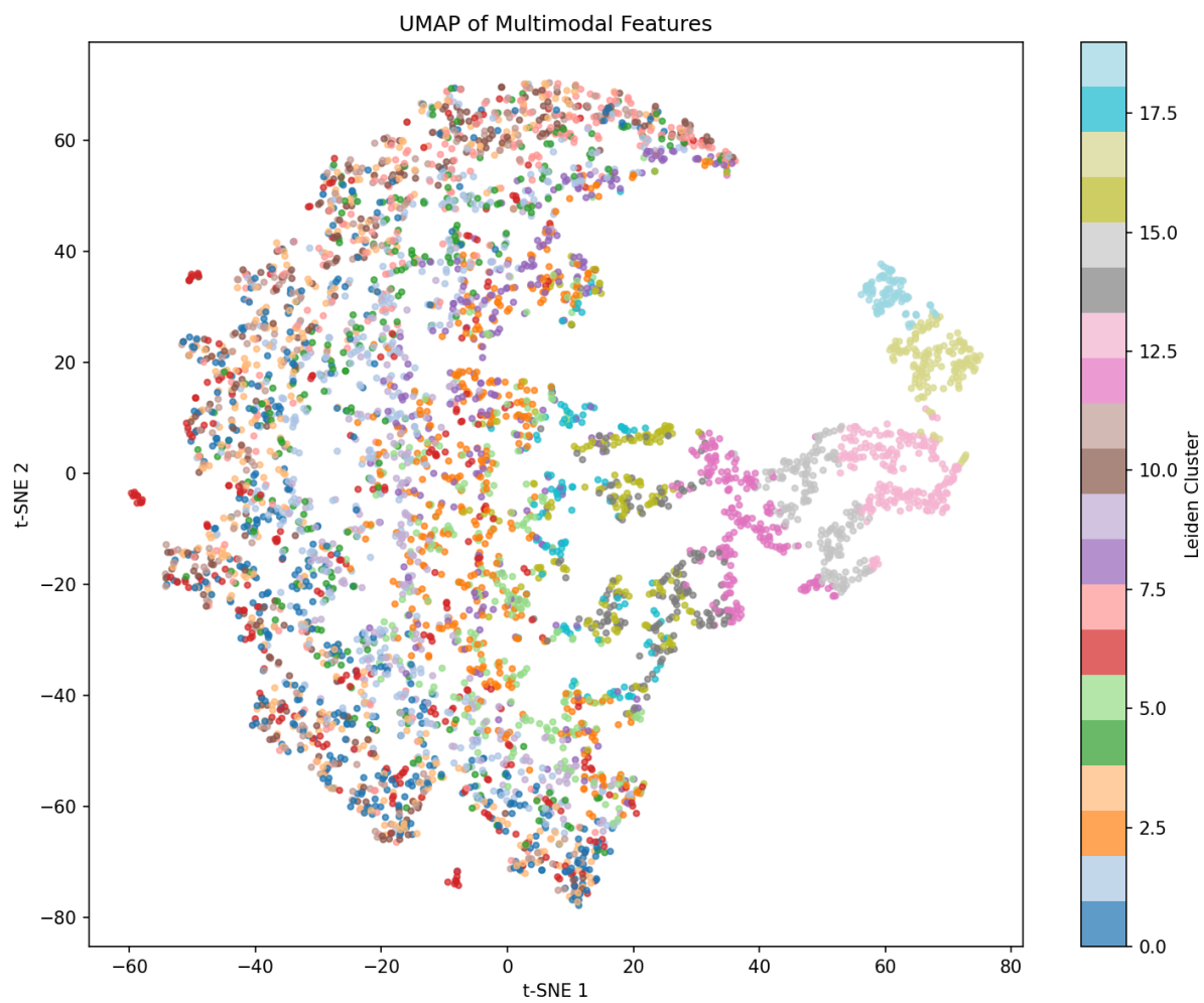
Figure 8: Feature Space UMAP
