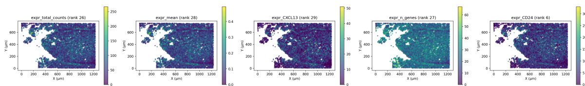
Figure 6: Top-5 Spatial Gene Expression
