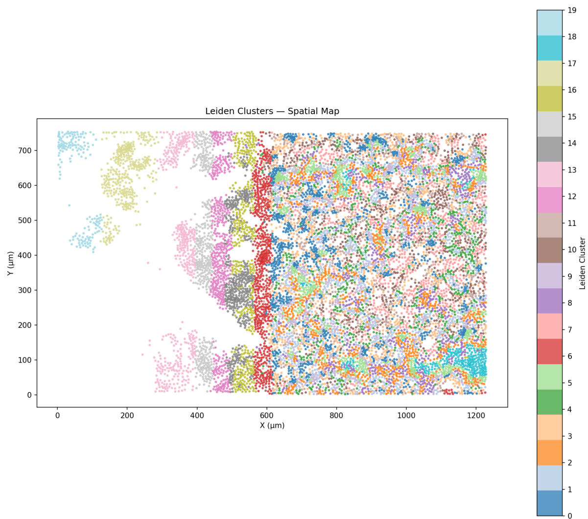
Figure 4: Spatial Clusters
