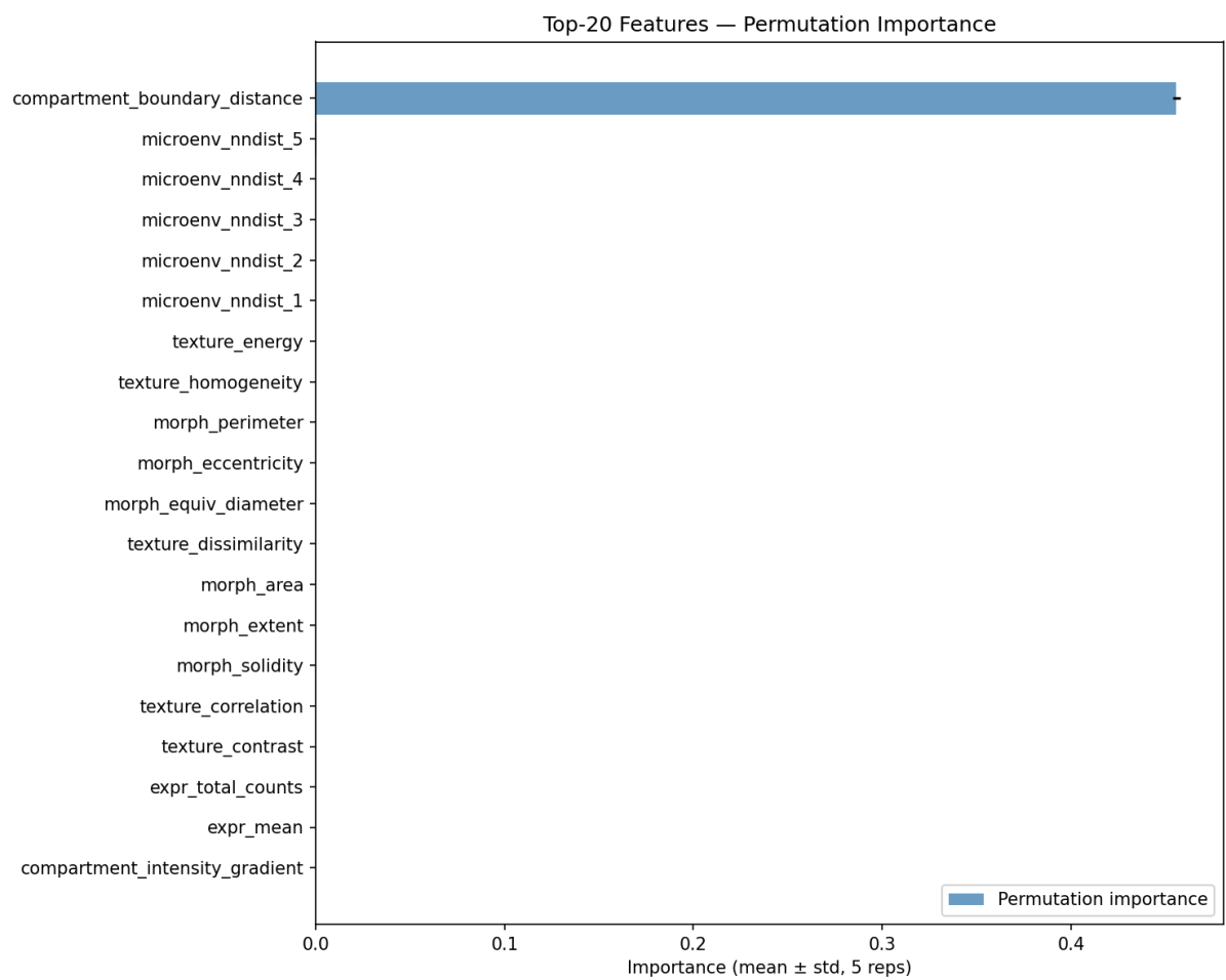
Figure 1: Top-20 Features
