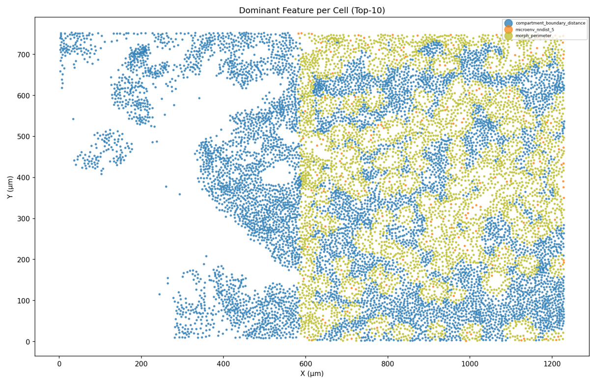
Figure 5: Dominant Feature per Cell
