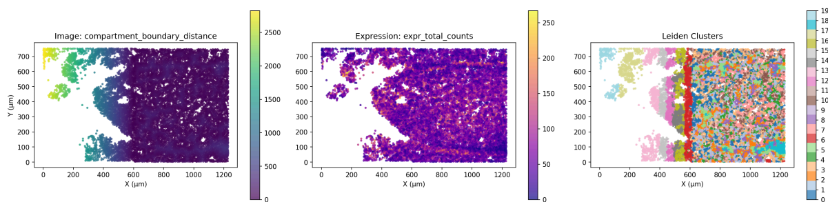
Figure 7: 3-Panel Comparison
