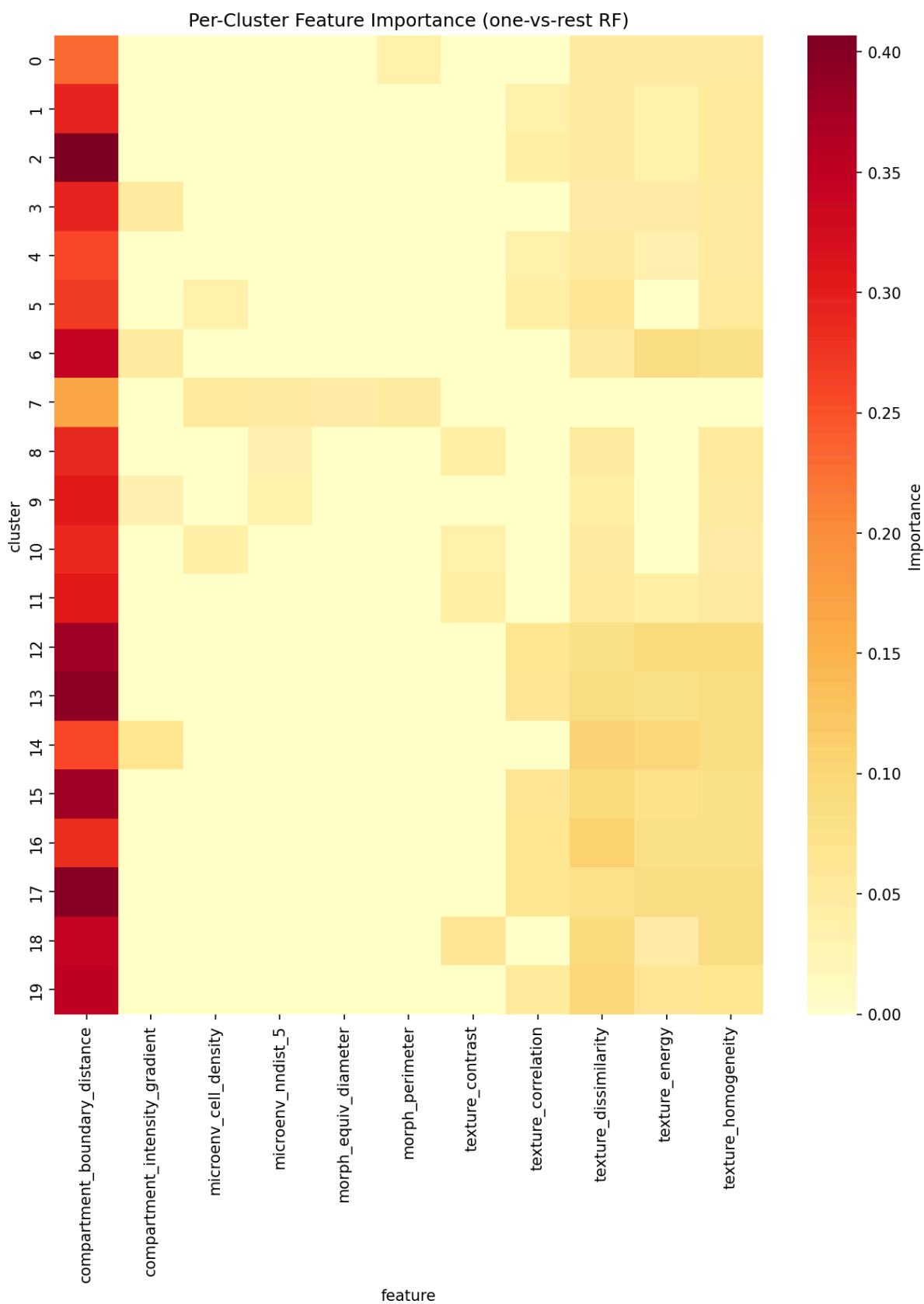
Figure 3: Per-Cluster Importance
