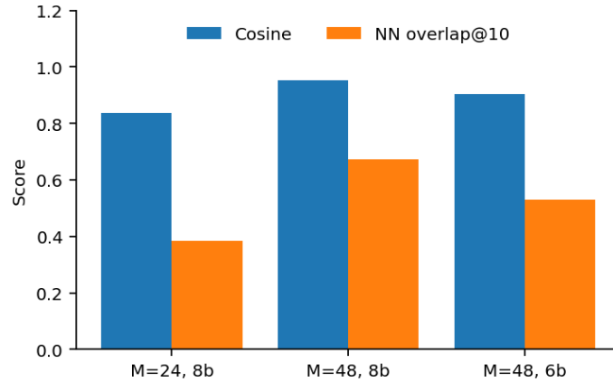
Figure 9: Public PQ codes preserve both vector direction and substantial nearest-neighbour structure in the rotated space.
