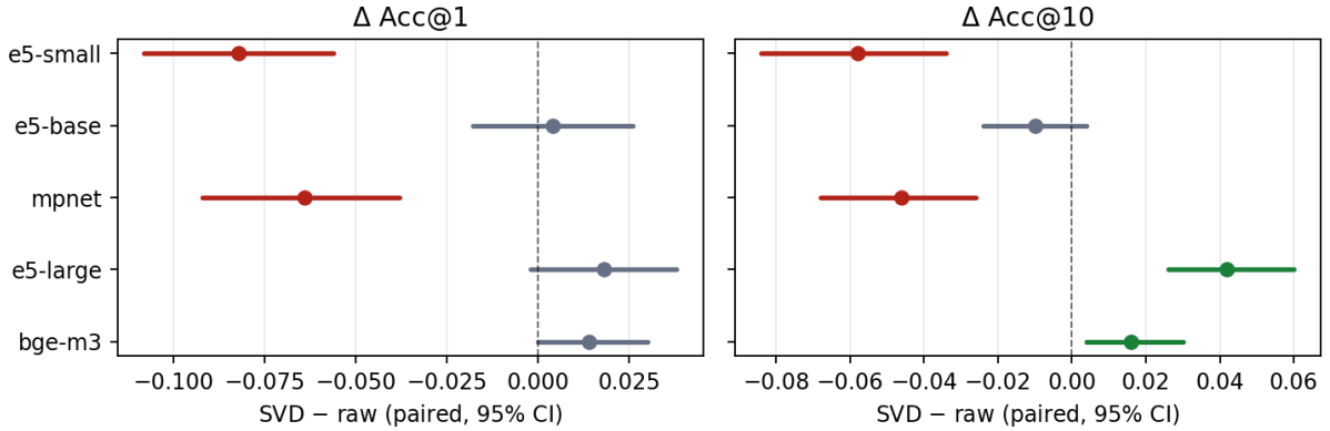
Figure 7: Paired effect of SVD truncation ( k = d/2 ) relative to the raw space, with bootstrap 95% CIs, on 500 self-retrieval queries. Green markers are significant improvements ( p < 0.05 , McNemar), red significant degradations, grey not significant. No encoder shows a significant Acc@1 gain; the significant Acc@10 gains are confined to the retrieval-trained d=1024 encoders.
