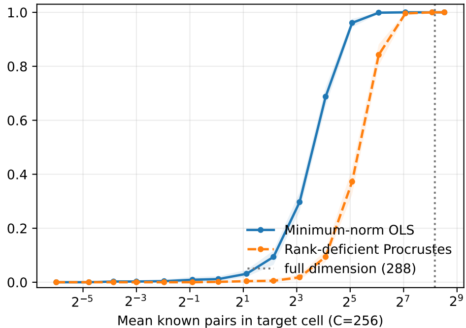
Useful recovery precedes full rank
