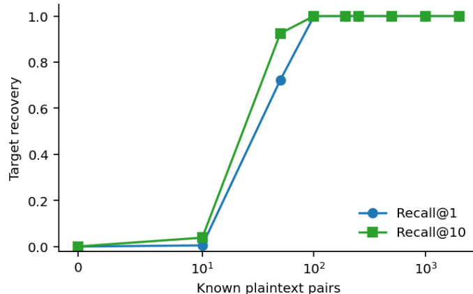
Figure 2: Known-plaintext alignment quickly destroys the unknown-rotation assumption. The x axis uses a symlog scale to include m = 0 .
