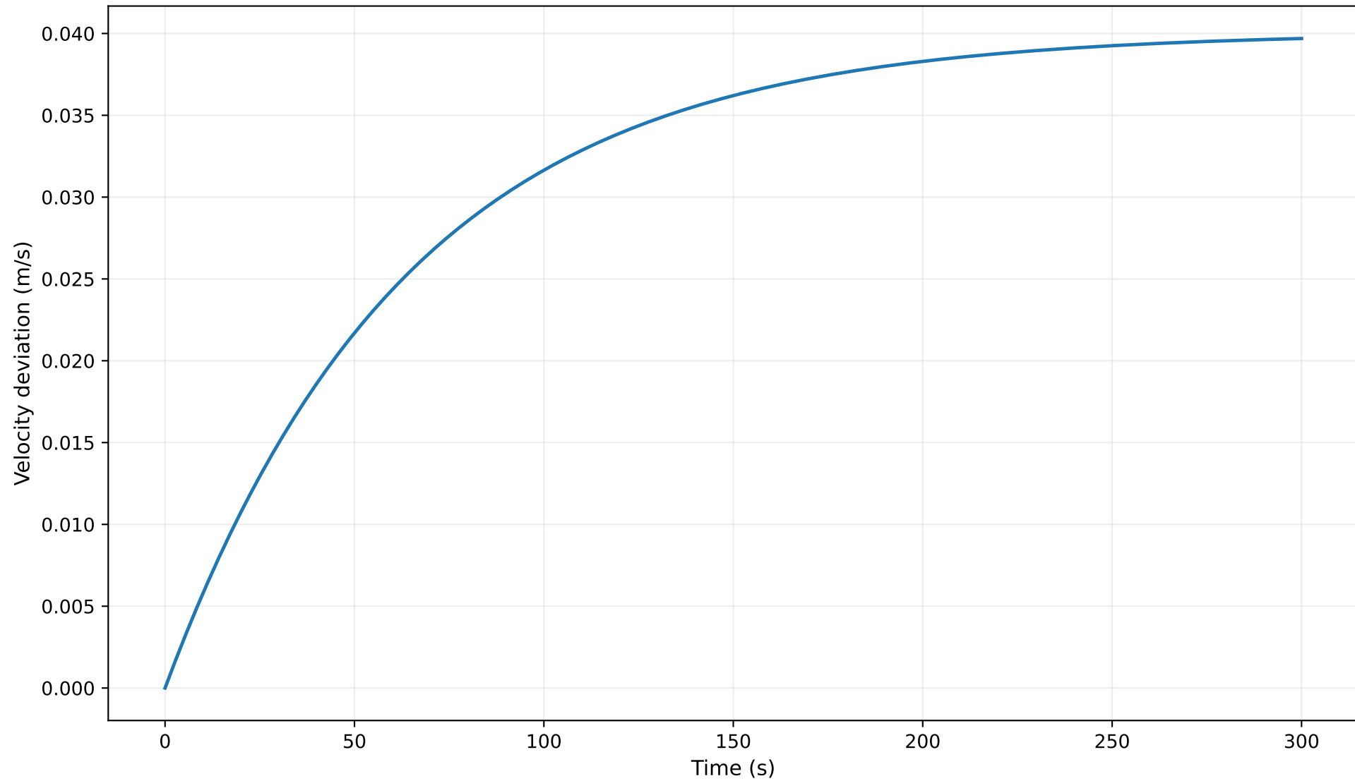
Open-loop step response
