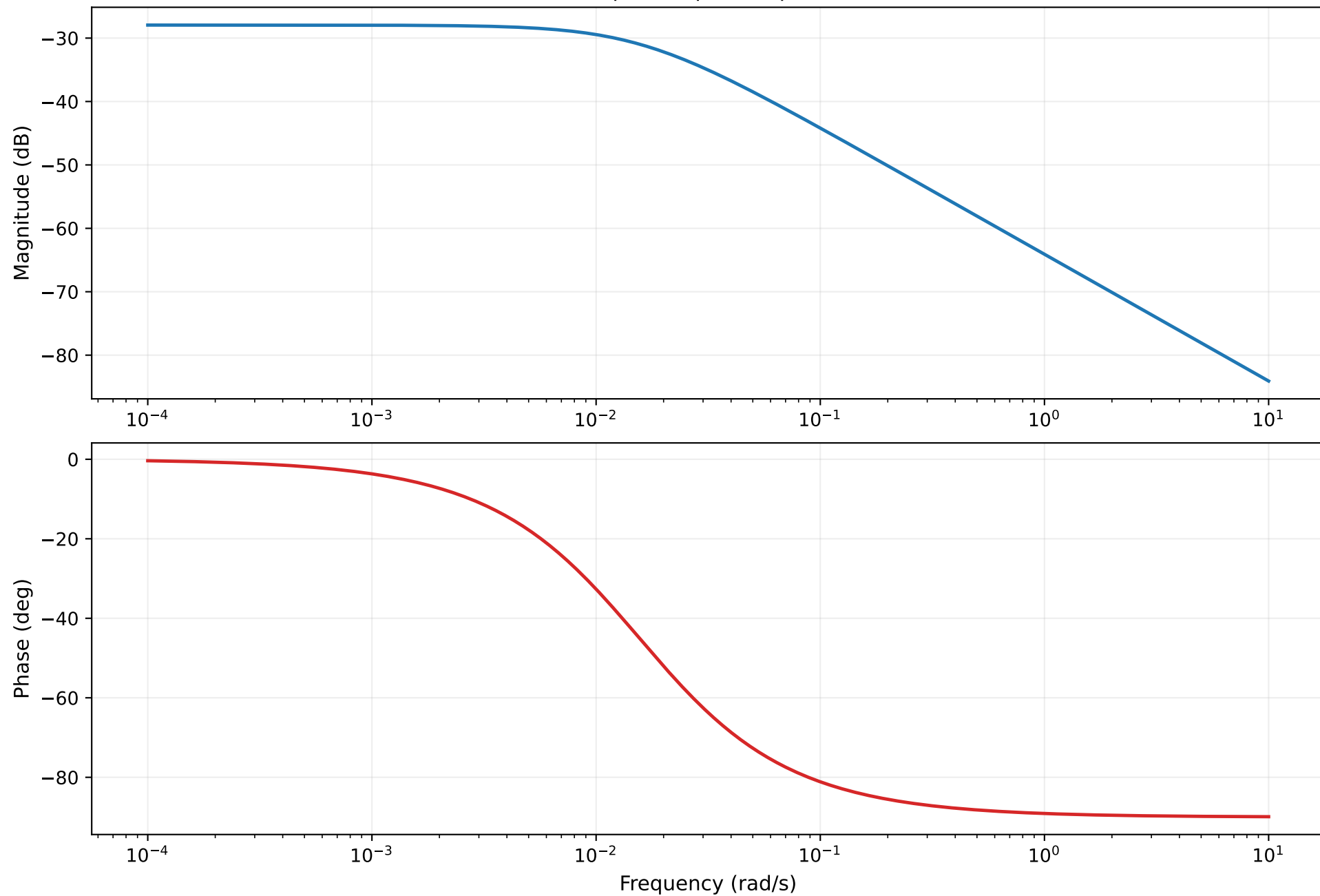
Open-loop Bode plot
