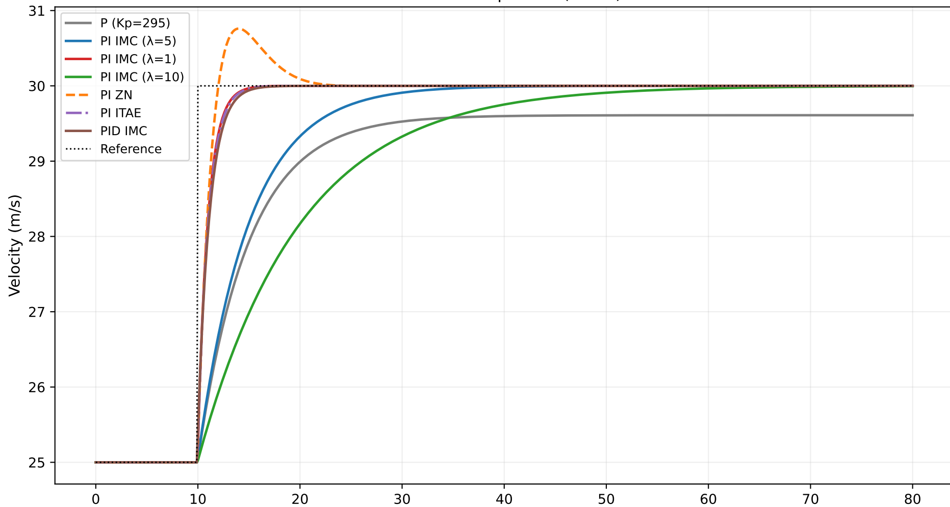
S1 servo comparison (linear)
