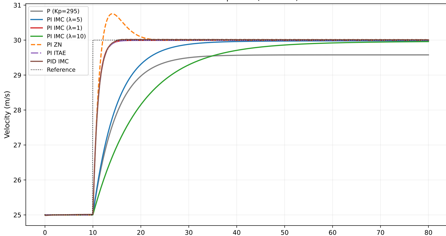
S1 servo comparison (nonlinear)
