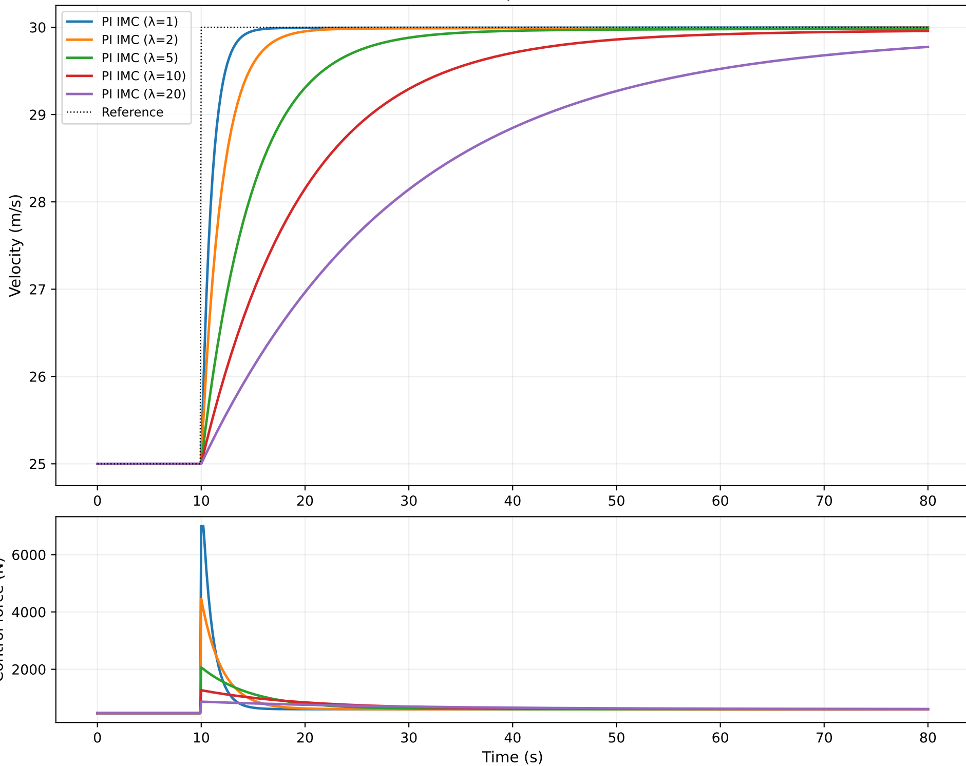
IMC \lambda sweep (nonlinear)
