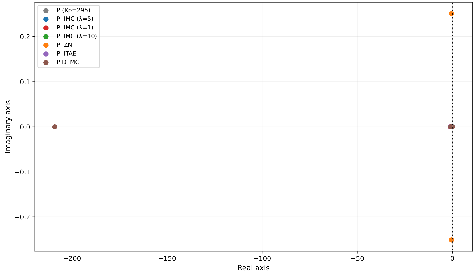
Closed-loop pole map
