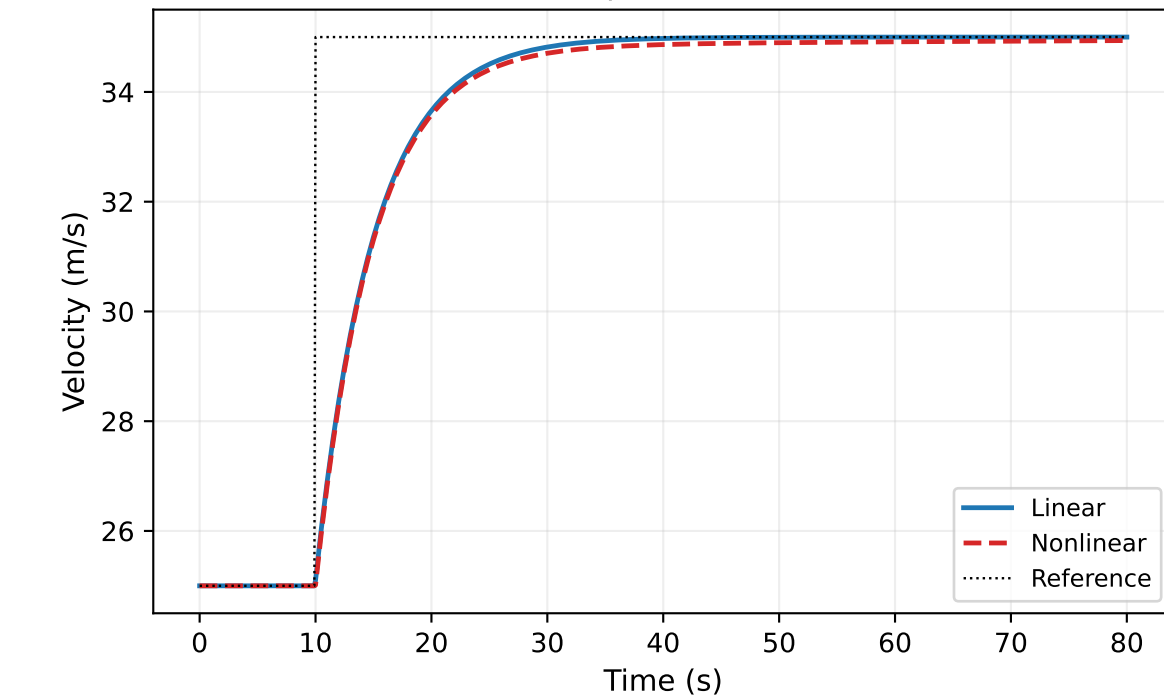
Step +10 m/s
