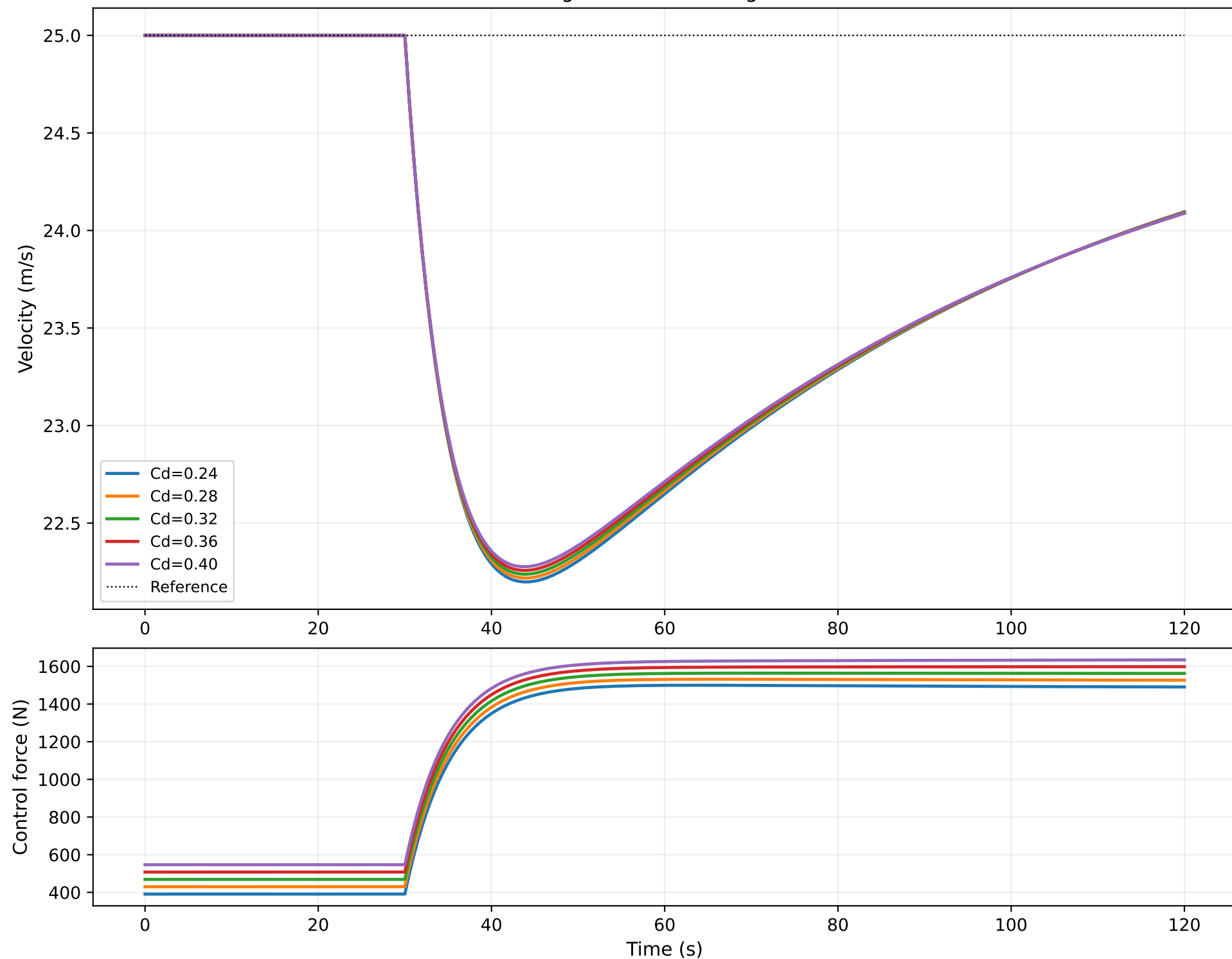
Drag variation under grade
