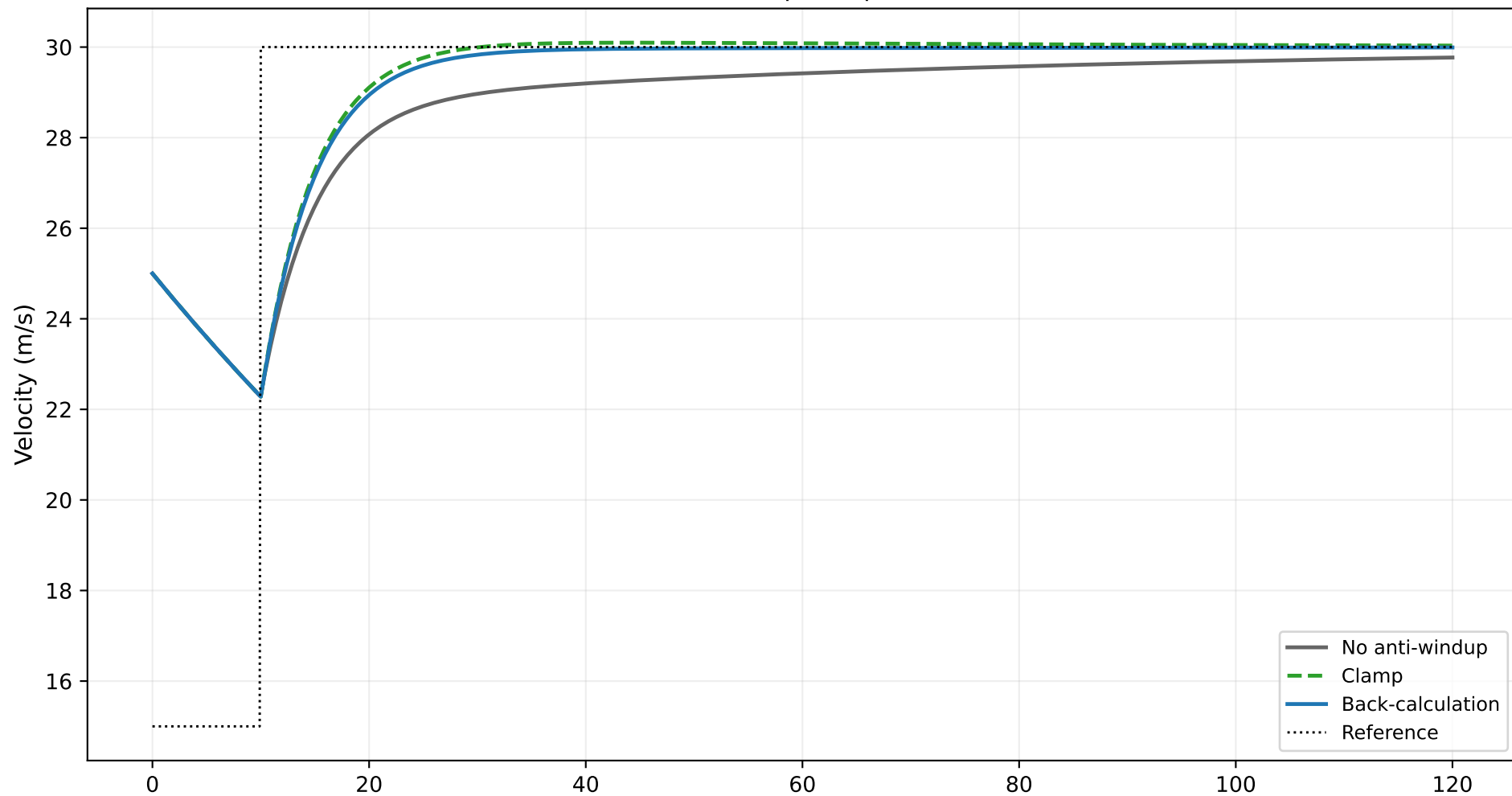
Anti-windup comparison
