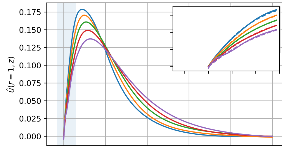
PINN simulations
