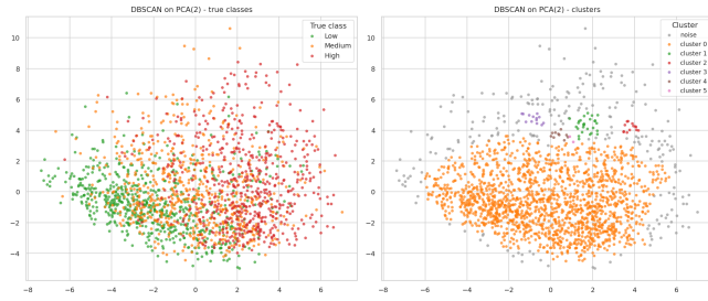
FIGURE 13. DBSCAN ( \epsilon = 0.5 , \text{minPts} = 10 ) on (PC1, PC2). The bulk of the data collapses into one dominant dense cluster (plus a few tiny fringe clusters), with 233 samples (12.3%) flagged as noise.
