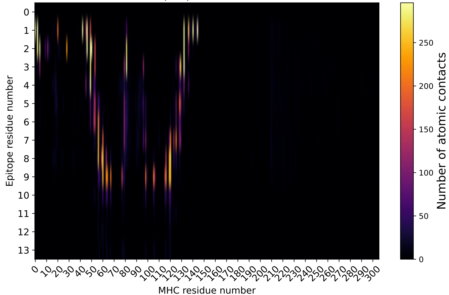
MHC-Epitope contact counts
